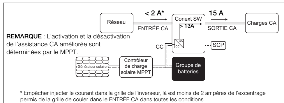
Figure 1-4 Assistance CA améliorée
