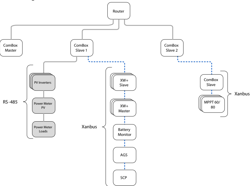
Figure 3-5 Example Master-slave Configuration
